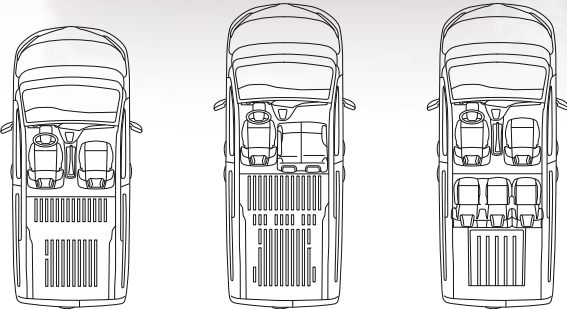
Short wheelbase
